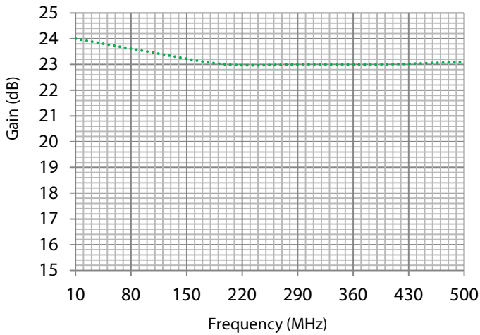
Gain (dB)
